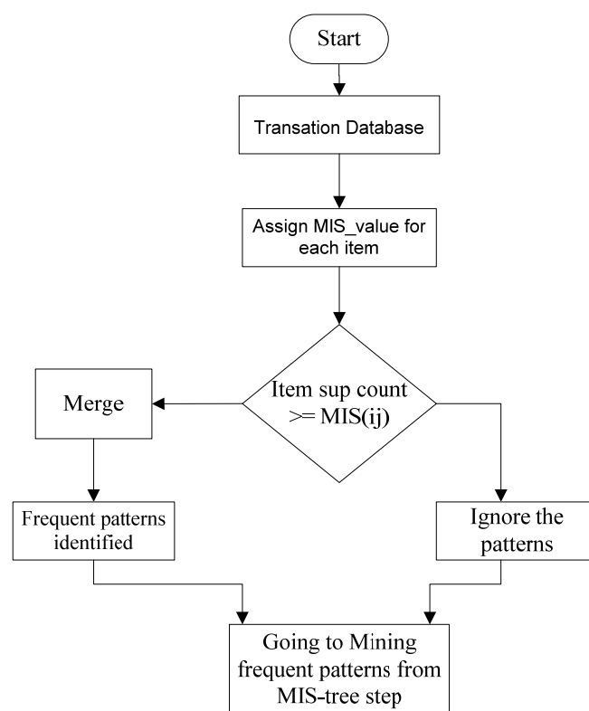
Fig. 1 Flow Diagram of MIS-Tree
