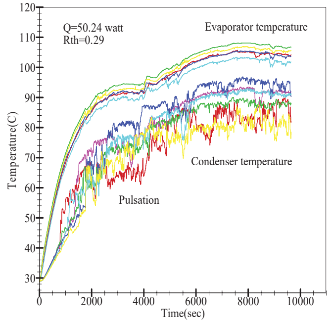
Fig. 4 Evaporator and condenser temperatures at 50.24 Watt
