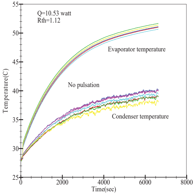
Fig. 3 Evaporator and condenser temperatures at 10.53 Watt
