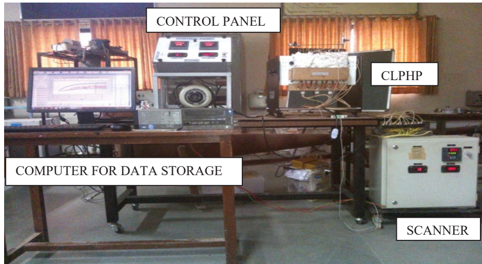
Fig. 1 CLPHP experimental setup
