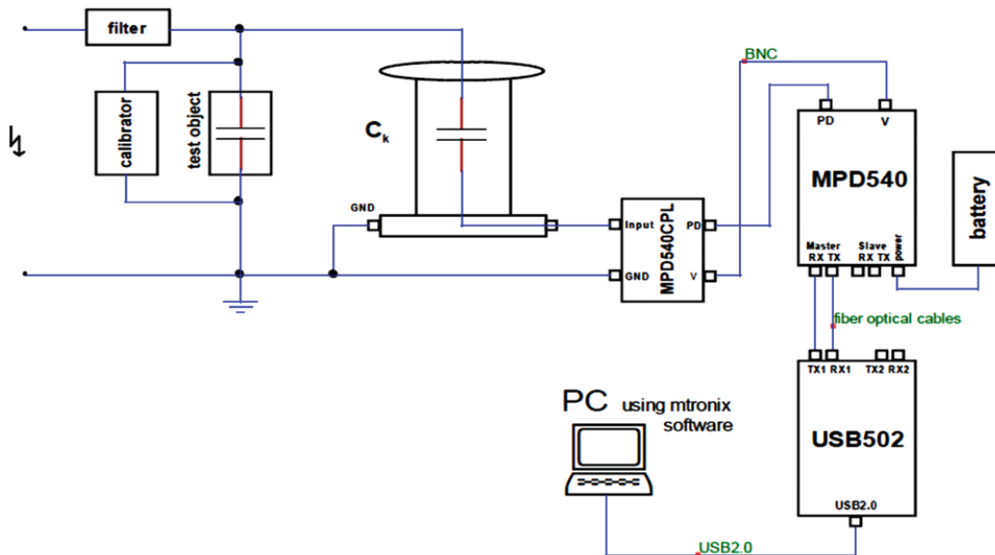
Fig. 4 Measurement circuit for PD Measurement system
