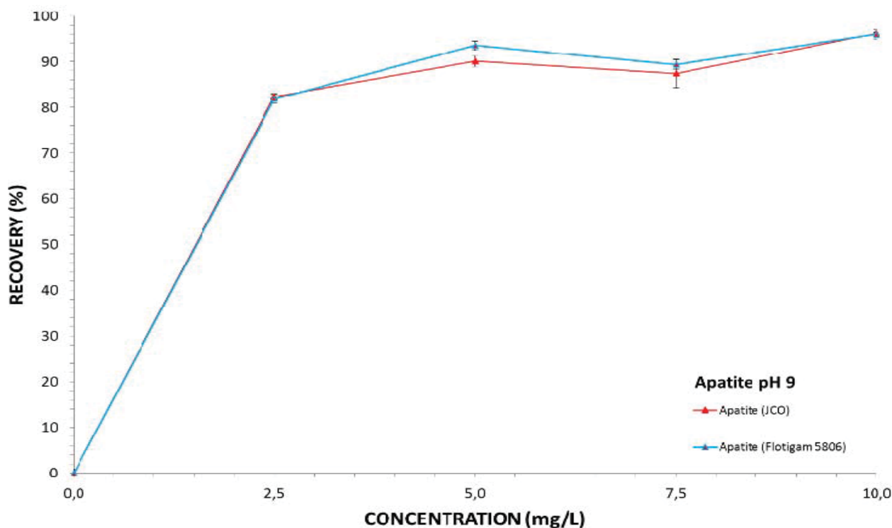
Fig. 4 Apatite recovery variation with collectors' concentration (Flotigam and JCO) at pH 9
