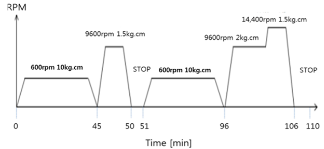
Fig. 2 The operating cycle profile of washing machine
