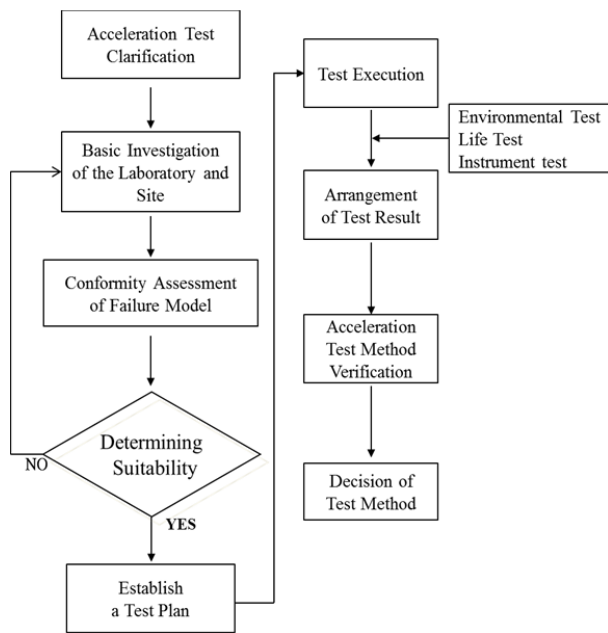
Fig. 1 Flow chart for accelerated life cycle test
