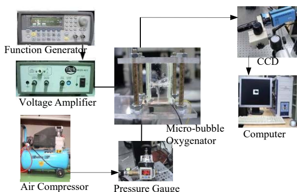
Fig. 5 Schematic diagram of experiment apparatus
