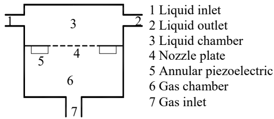
Fig. 1 Illustration of the micro bubble oxygenator
