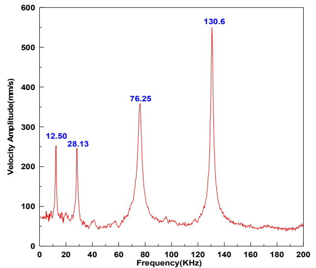
Fig. 3 Frequency response of the vibrating piezoelectric transducer
