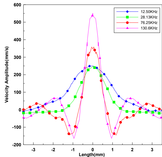
Fig. 4 Cross section profiles of mode shapes of vibrating piezoelectric transducer
