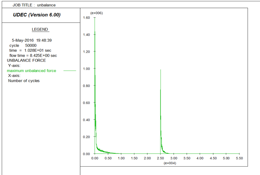
Fig. 5 Unbalanced forces
