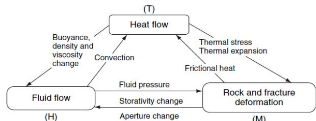
Fig. 1 Thermo-hydro-mechanical process in rock joints [2]
