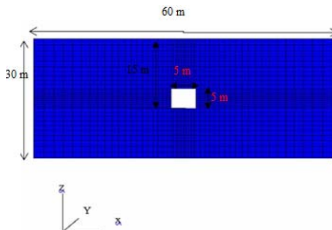
Fig. 2 Model geometry
