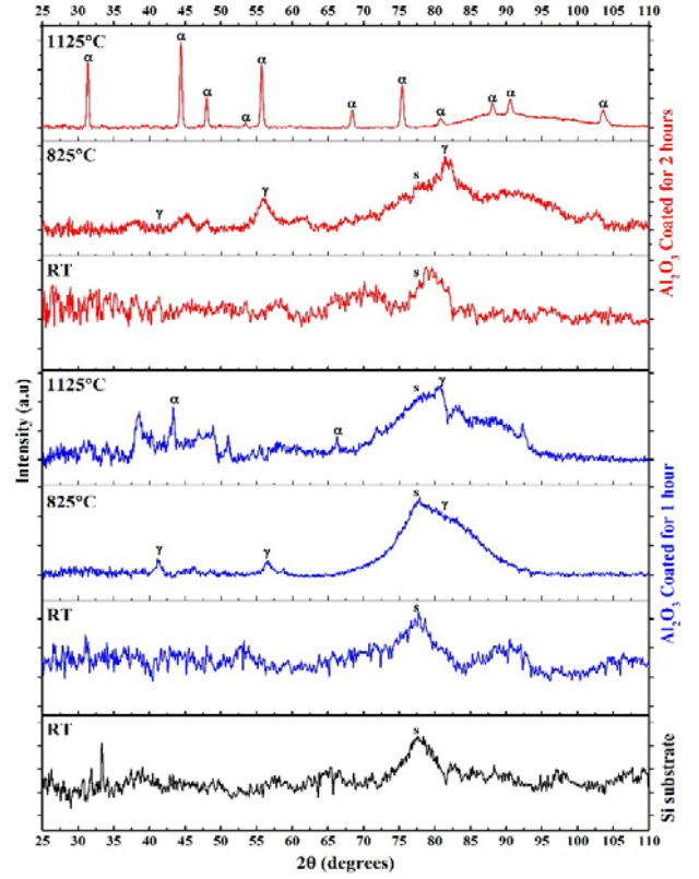
Fig. 2 XRD diffractograms of non-coated & Al_2O_3 coated (1 h & 2 h) Si substrates at room temperature (RT) and after annealing at 825 °C or 1125 °C (s: Si substrate, \alpha : \alpha - Al_2O_3 , \gamma : \gamma - Al_2O_3 )
