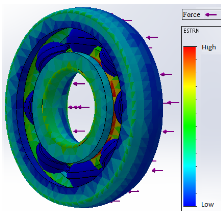
Fig. 4 Strain simulation
