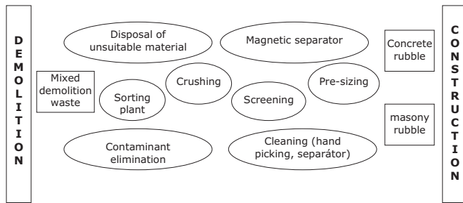
Fig. 3 Recycling process from demolition to material for new construction [4], [11]
