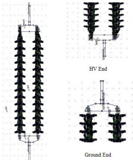
Fig. 1 220 kV porcelain double tension string model
