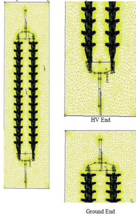
Fig. 2 Insulator model with 2D triangular elements
