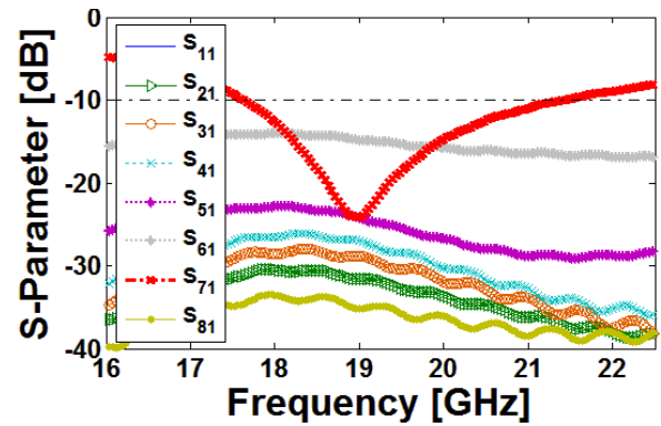
Fig. 9 S parameters of the designed 5G antenna
