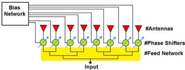
Fig. 8 Phased array architecture for the proposed array
