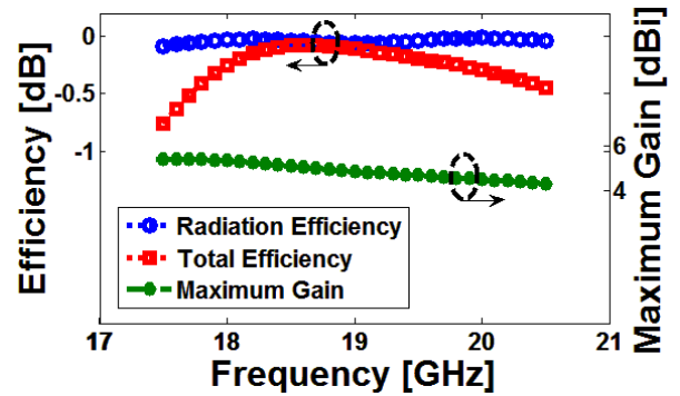
Fig. 6 Fundamental properties of the single-element antenna
