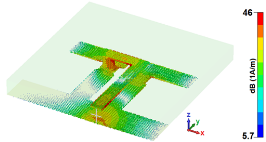
Fig. 4 Simulated current distribution at 19 GHz
