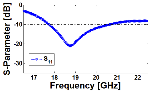
Fig. 3 S_{11} characteristic of the antenna
