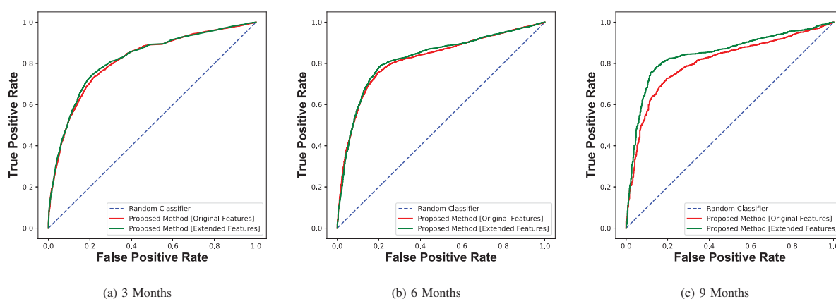
Fig. 4 ROC Curves
