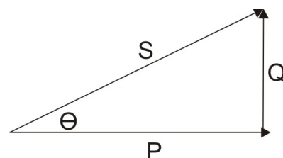
Fig. 1 Power triangle
