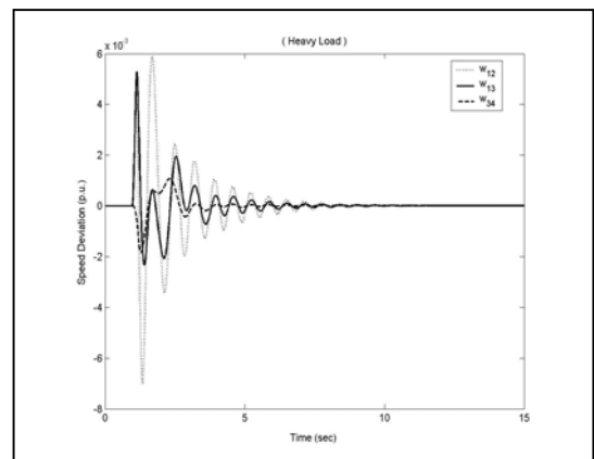
Fig. 10 Dynamic response for \Delta\omega_{12} , \Delta\omega_{34} , \Delta\omega_{13} considering transitory 3-phase fault at bus-7 of three cycles duration for heavy loading conditions with GFLPSS
