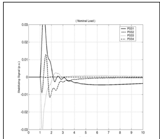
Fig. 14 Stabilizing signal under small perturbation with GFLPSS
