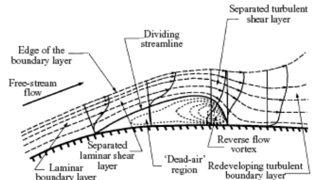
Fig. 1 Structure of a laminar separation bubble
