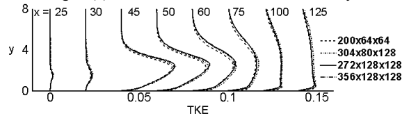
Fig. 4 (b) Profiles of TKE
