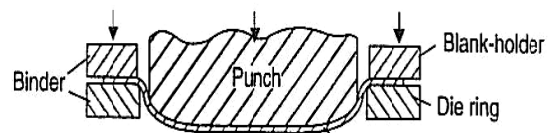
Fig. 1 Schematic of Mechanical forming process [4]
