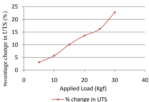
Fig. 8 Graph of percentage change in UTS
