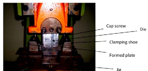
Fig. 2 Experimental set-up for mechanical bending process
