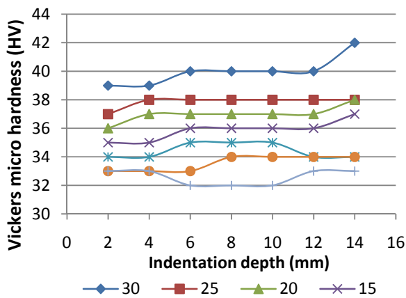
Fig. 5 Plots of Vickers microhardness against depth
