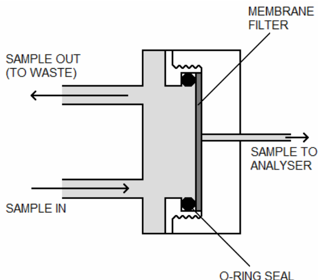
Fig. 4 Schematic cross section of the sampling port. The threaded parts of the membrane holder are screwed together so that the membrane is held in place by the O-ring seal. Sample circulates past the outer side of the membrane and the required volume is drawn into the analyser by a solenoid pump
