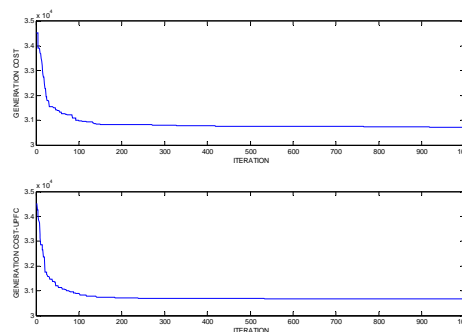
Fig. 9 Iteration Vs Cost Curve
