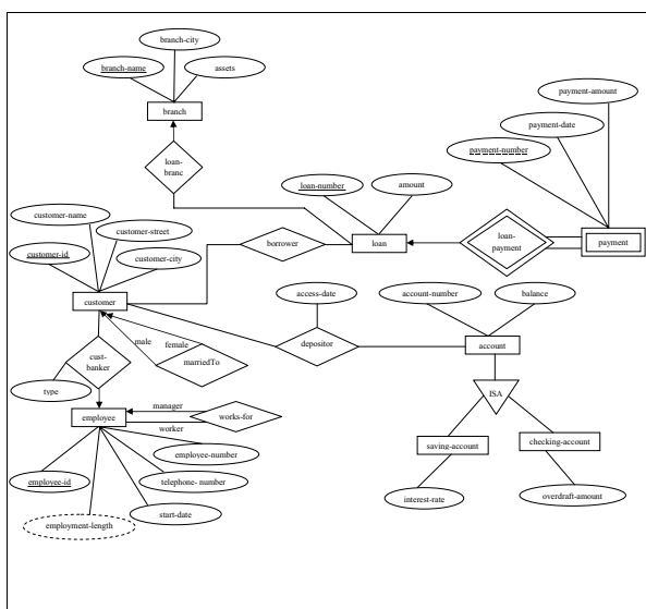
Fig. 1. E-R diagram for a banking enterprise
