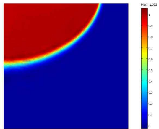
Fig. 6 : Martensite distribution after cooling ( t=20s )
