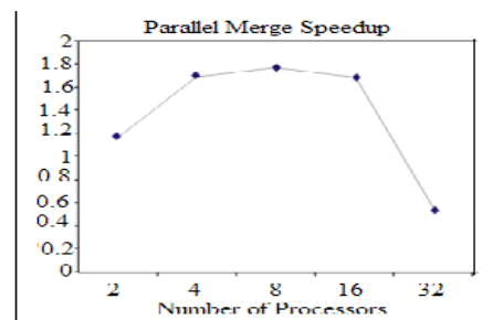
Fig. 9 Speedup of the Parallel Merge Sort Algorithm
