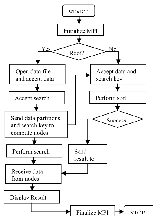
Fig. 1 Parallelization of Sorting Algorithms
