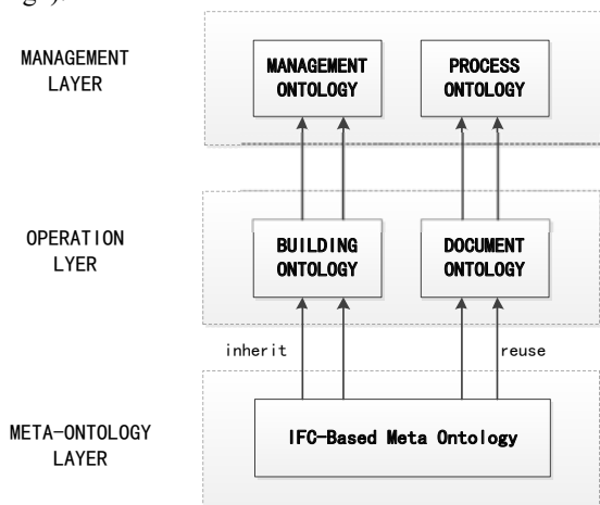
Fig. 2 IFC-based construction domain ontology framework
