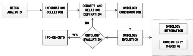
Fig. 1 IFC-CE-Onto construction method
