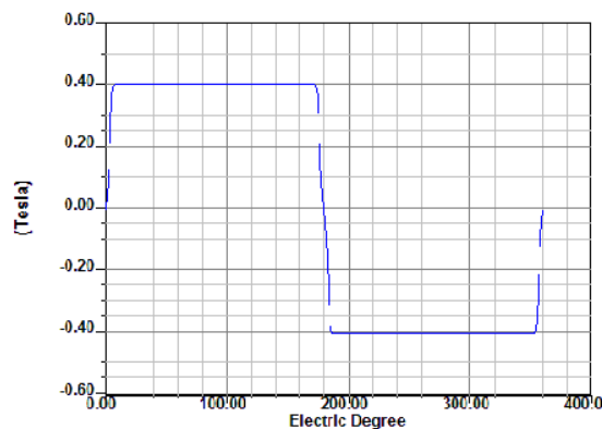
Fig. 6b Air gap flux versus electrical degree
