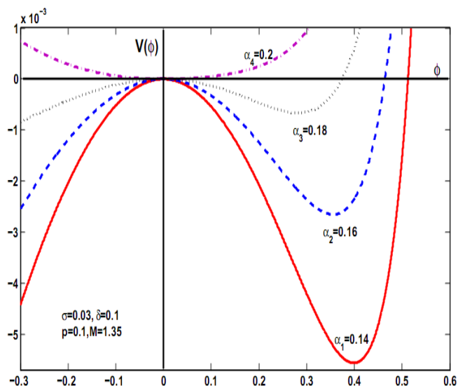
Fig. 1 The Sagdeev potential V(\phi) with respect to \phi for fixed value of \sigma=0.03 , p=0.1 , \delta=0.1 , M=1.35 and different values of \alpha
