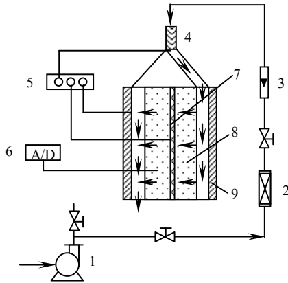
Fig. 1 Experimental flow sheet
