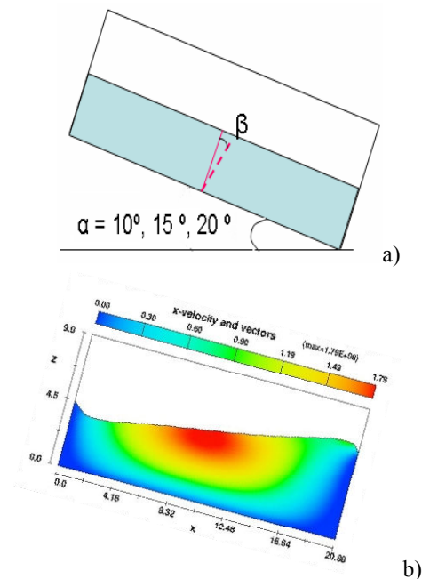
Fig. 1 Experimental single fiber motion in viscous flow: a) experiment; b) viscous fluid flow velocity (along the container) modeling result (FEM code Flow 3D simulation)
