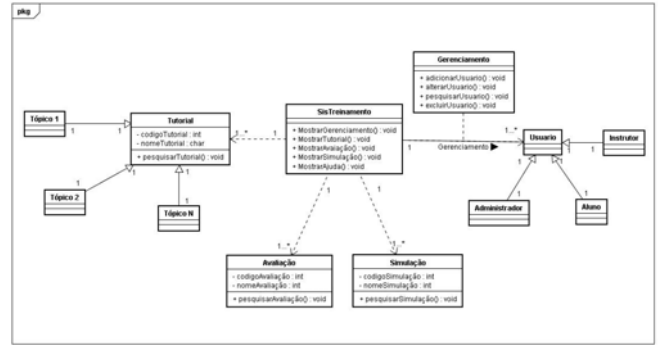
Fig. 9 Class diagram
