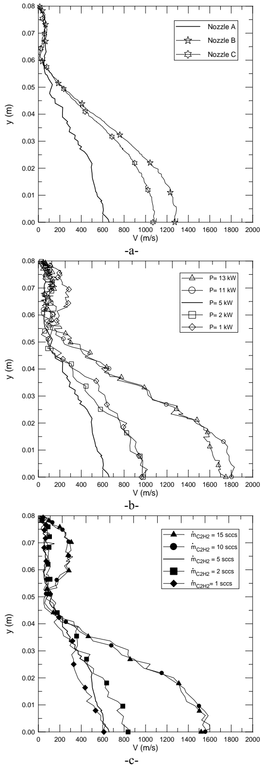
Fig. 10 Profiles of velocity along the radius of the chamber at x=0.2 m by nozzle A, B and C (a), by different electrical power (b) and by different mass flow rate of C_2H_2 (c)
