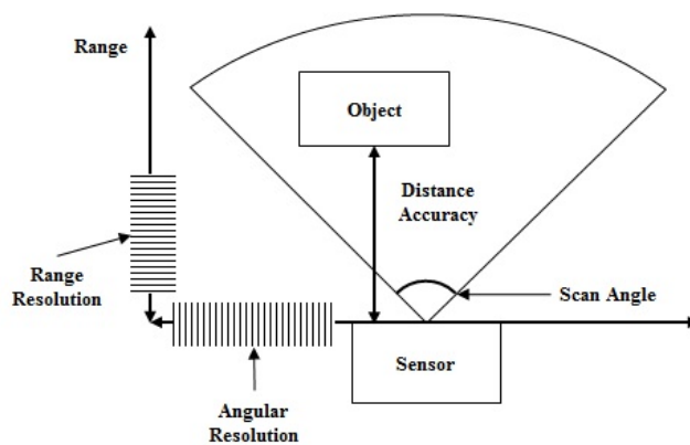
Fig. 1 Sensor Specification
