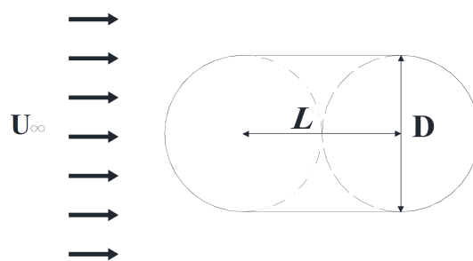
Fig. 1 Solution domain
